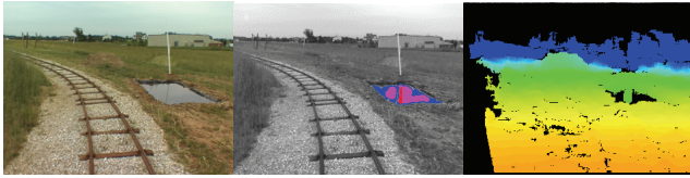
Figure 10. A frame showing the first man-made water body on the test course described in Figure 9 during a 1m/s run (left), water detection results overlaid on a grayscale intensity image (middle), and a wide-baseline stereo range image (right). In the color coded water detection overlay, blue, magenta, and red correspond to one, two, and three cues for water, respectively. In the stereo range image, black corresponds to no range data.
